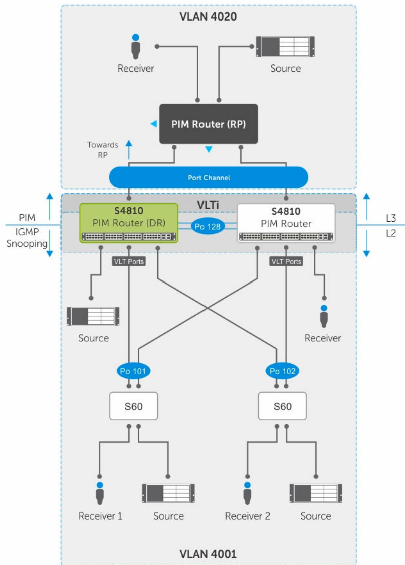
Figure 120. PIM-Sparse Mode Support on VLT
